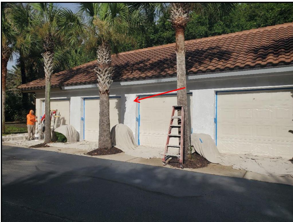
Photograph 9. Standalone garage primer coating application in progress.
