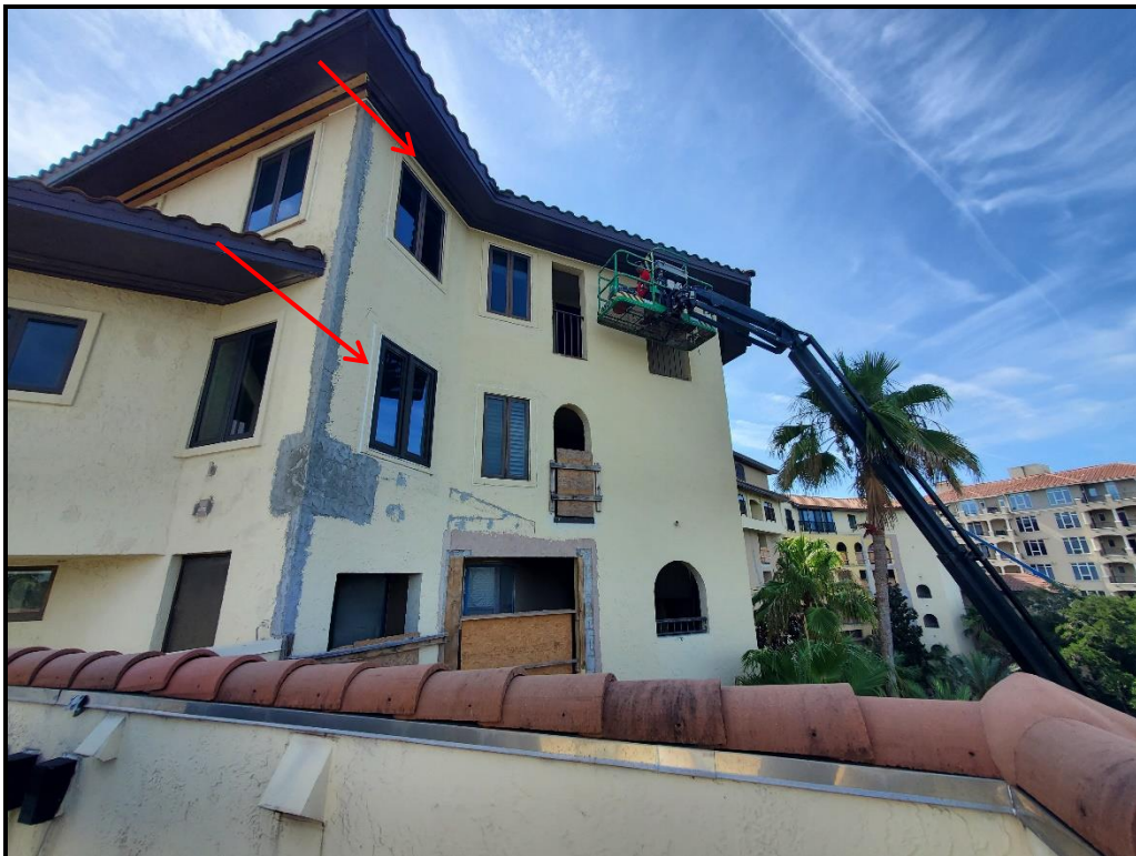
Photograph 17. West elevation new sealant application in progress on soffit and window stucco bands.
